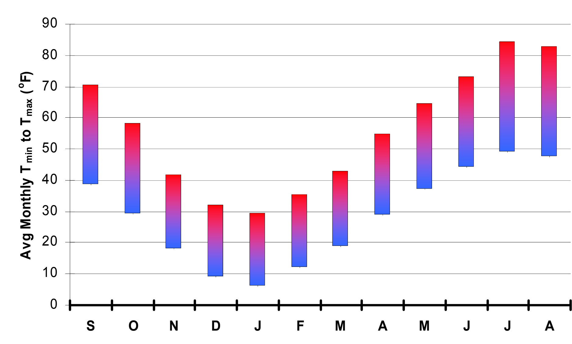
Figure 2. 1971-2000 average monthly minimum and maximum temperatures, September-August, at Amsterdam, MT.
